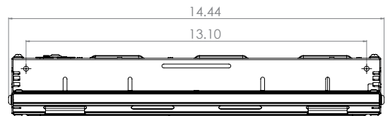
Side View: 12000LM, 15000LM, 18000LM MVOLT
