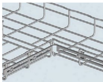
99642 Cablofil Legrand EZF90EZ 90° Bend and T Kit [99642]
